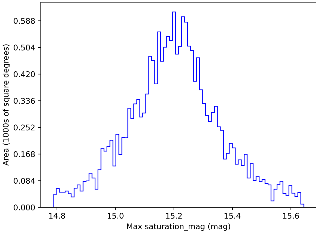
too_elab_r8_d2_griz_v3.4_10yrs WFD z band: Max saturation_mag
