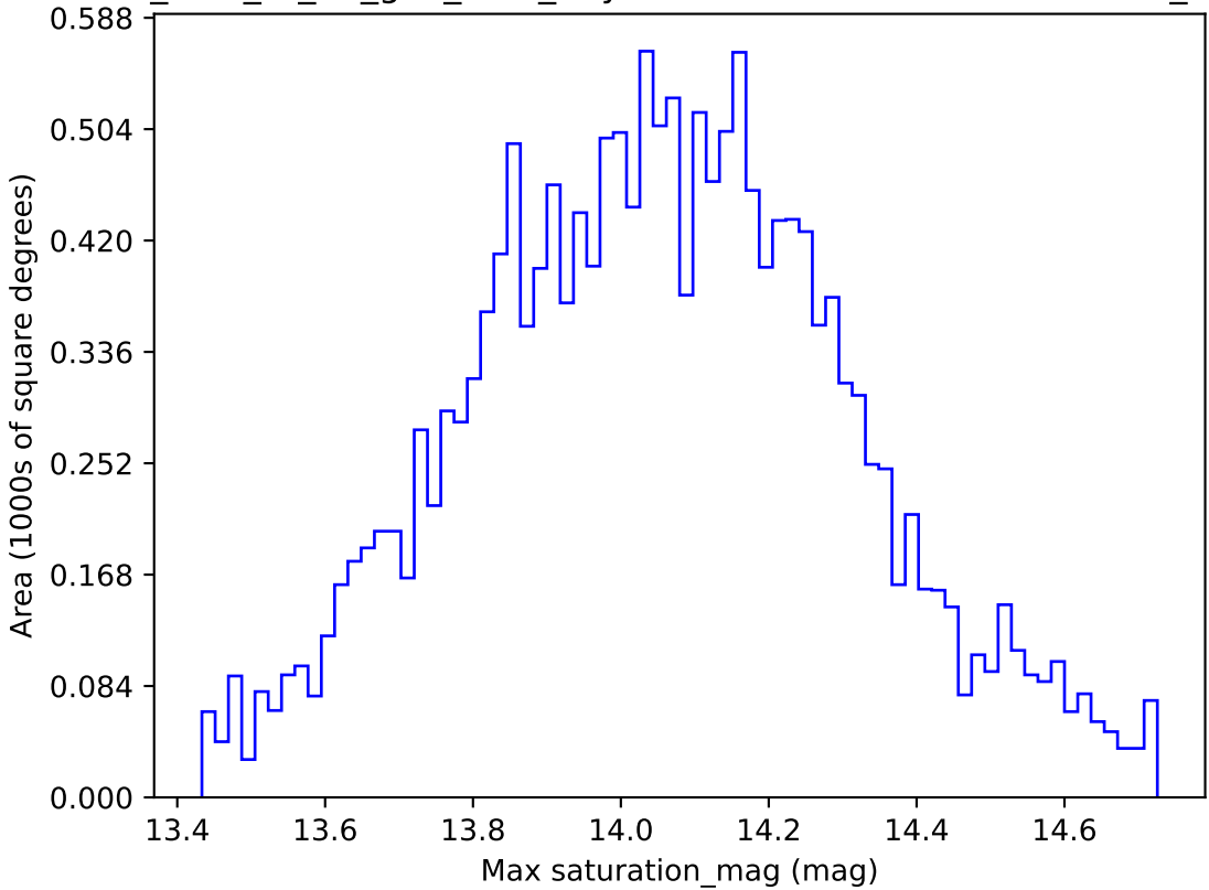
too_elab_r8_d2_griz_v3.4_10yrs WFD u band: Max saturation_mag
