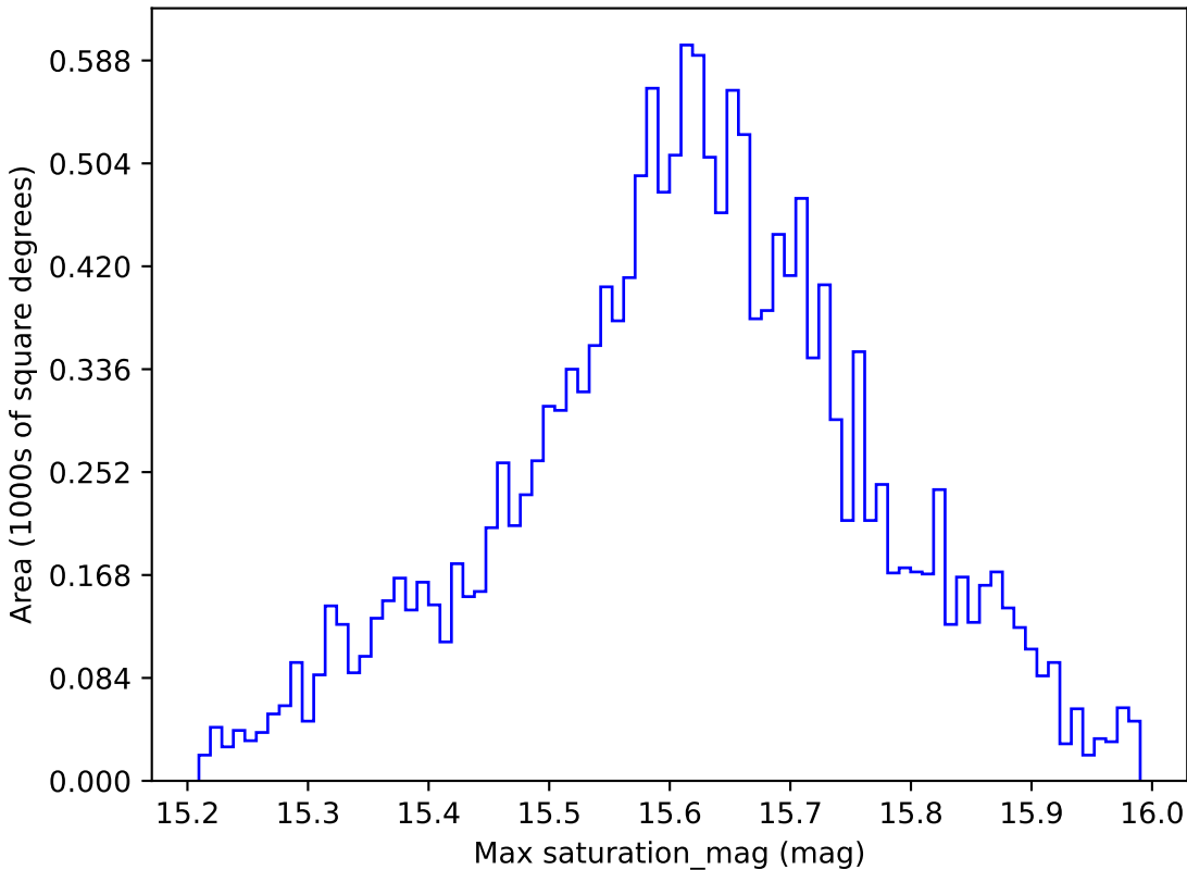
too_elab_r8_d2_griz_v3.4_10yrs WFD i band: Max saturation_mag
