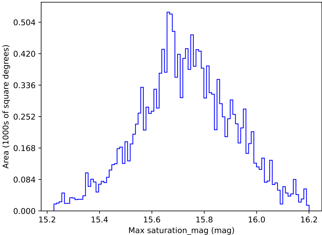
too_elab_r8_d2_griz_v3.4_10yrs WFD g band: Max saturation_mag
