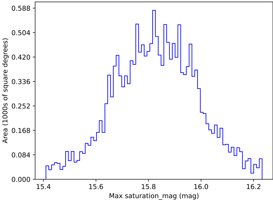
too_elab_r8_d2_griz_v3.4_10yrs WFD all bands: Max saturation_mag
