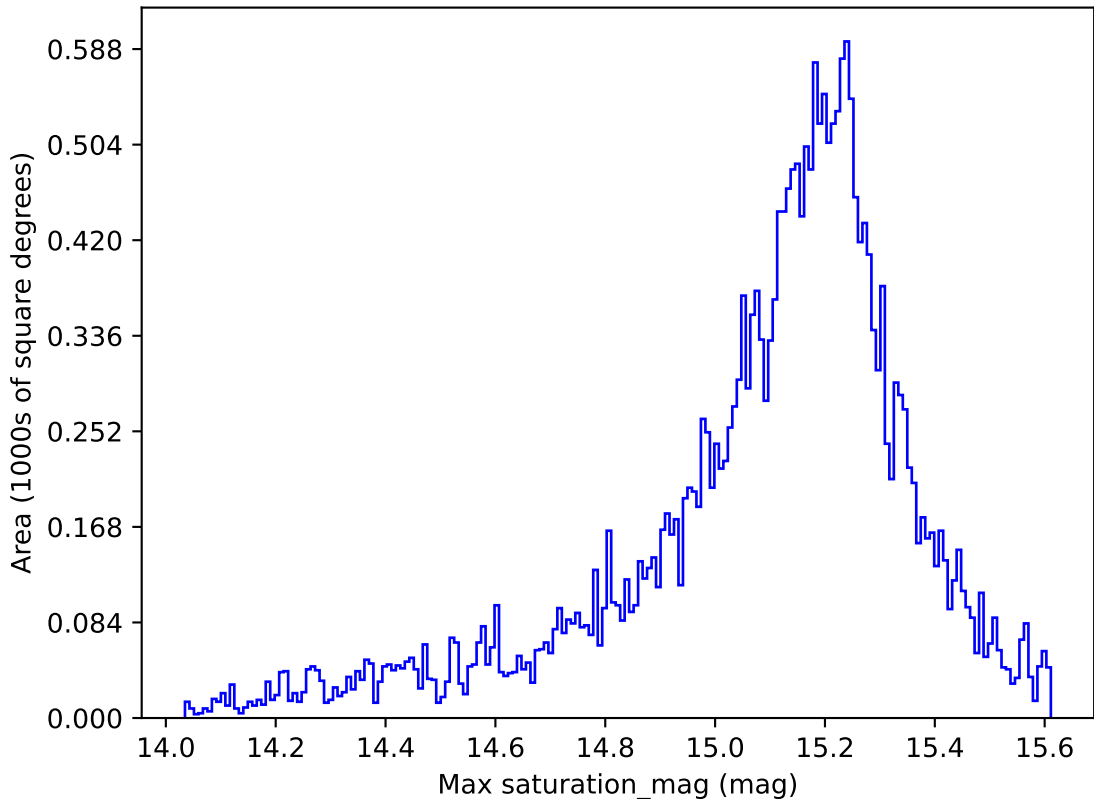
too_elab_r8_d2_griz_v3.4_10yrs All sky z band: Max saturation_mag
