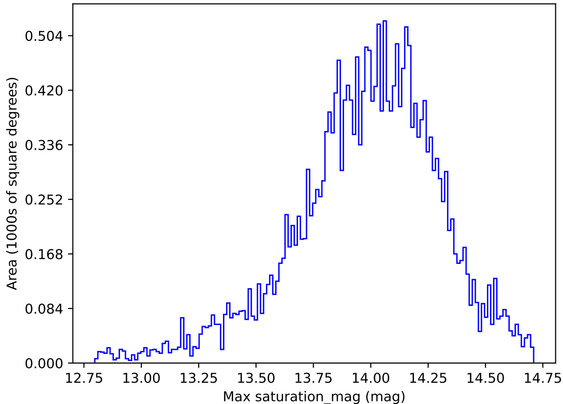
too_elab_r8_d2_griz_v3.4_10yrs All sky u band: Max saturation_mag
