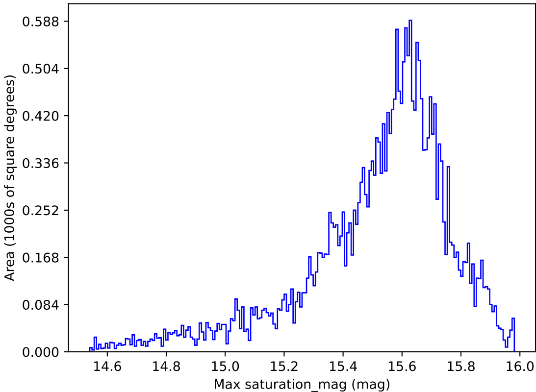
too_elab_r8_d2_griz_v3.4_10yrs All sky i band: Max saturation_mag
