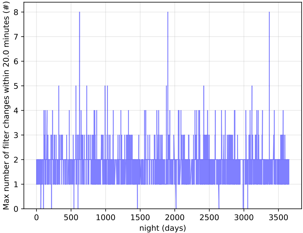
too_elab_r8_d2_griz_v3.4_10yrs Per Night: Max number of filter changes within 20.0 minutes
