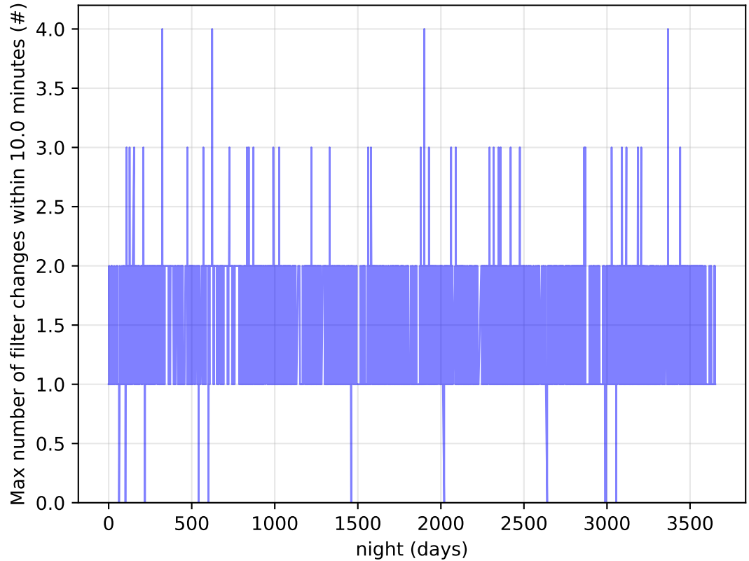
too_elab_r8_d2_griz_v3.4_10yrs Per Night: Max number of filter changes within 10.0 minutes
