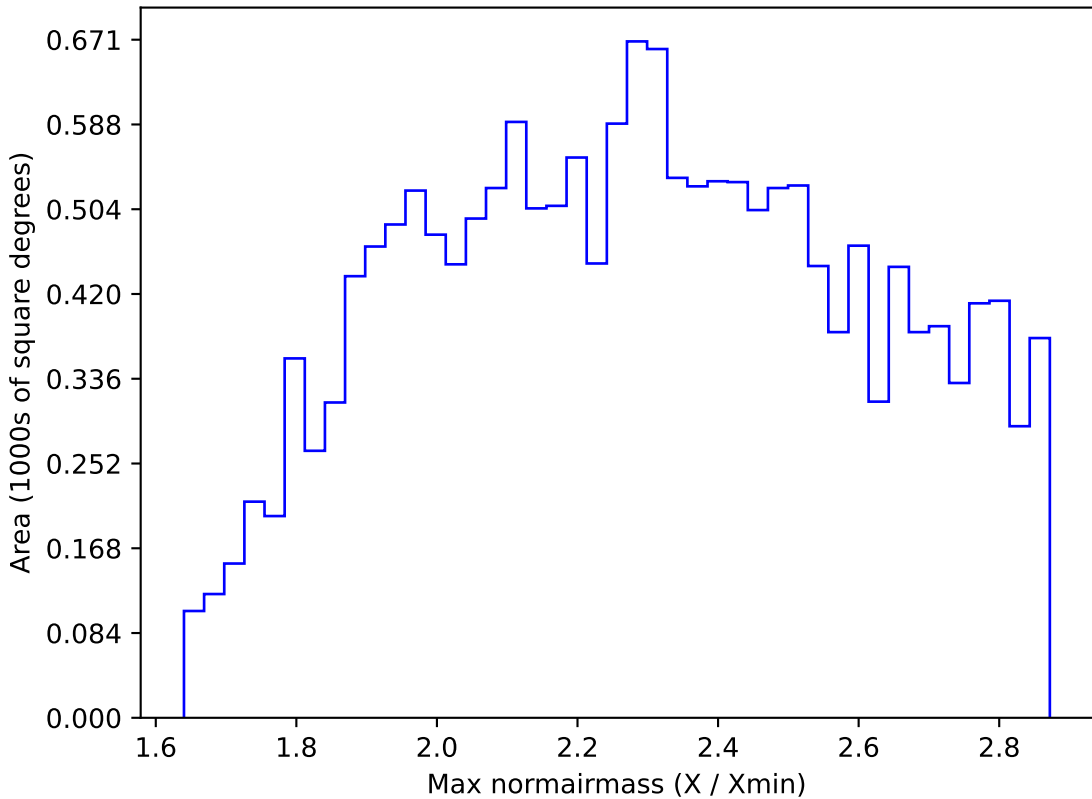
too_elab_r8_d2_griz_v3.4_10yrs WFD z band: Max normairmass
