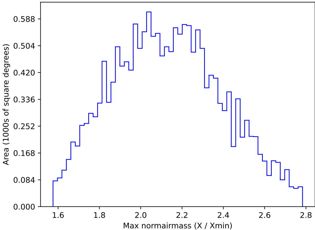
too_elab_r8_d2_griz_v3.4_10yrs WFD y band: Max normairmass
