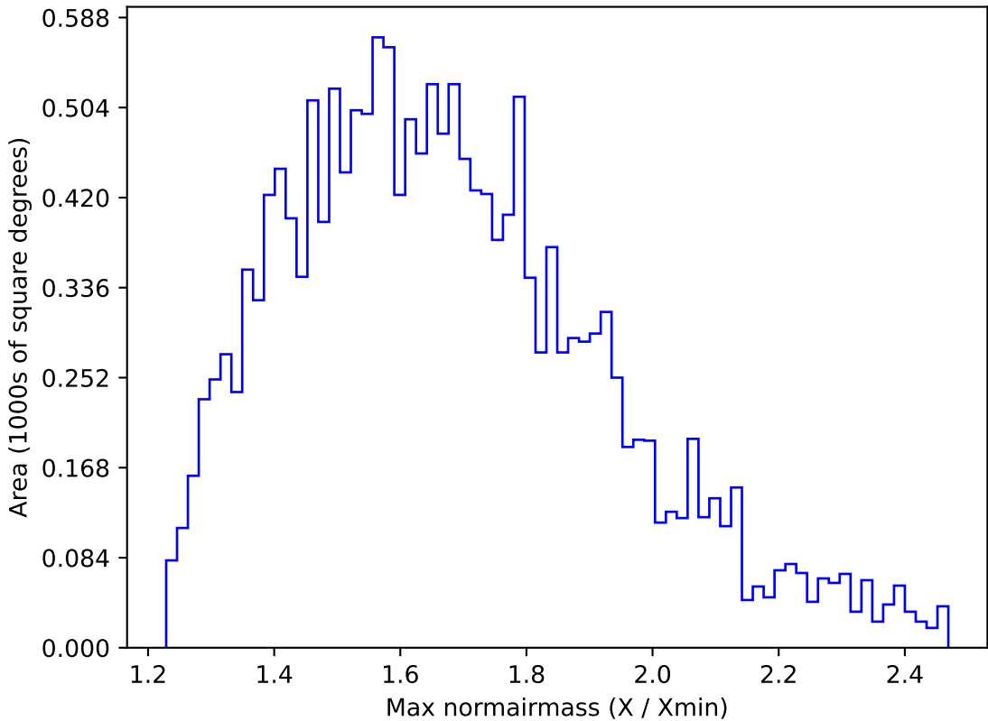
too_elab_r8_d2_griz_v3.4_10yrs WFD u band: Max normairmass
