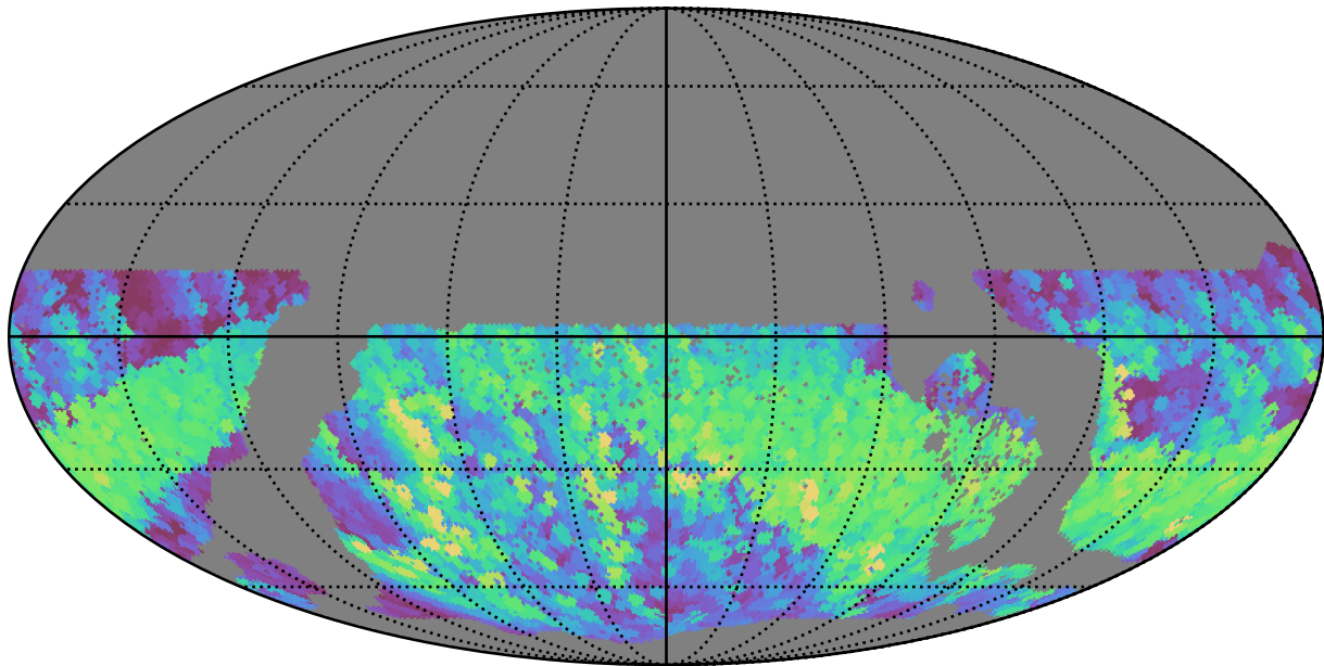
too_elab_r8_d2_griz_v3.4_10yrs WFD r band: Max normairmass
