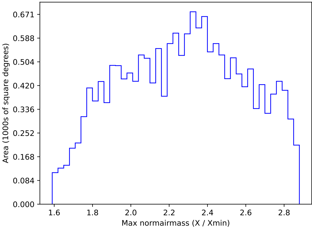
too_elab_r8_d2_griz_v3.4_10yrs WFD i band: Max normairmass
