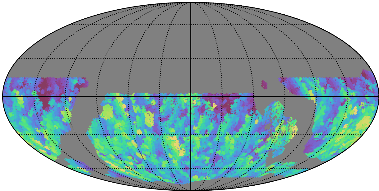
too_elab_r8_d2_griz_v3.4_10yrs WFD g band: Max normairmass
