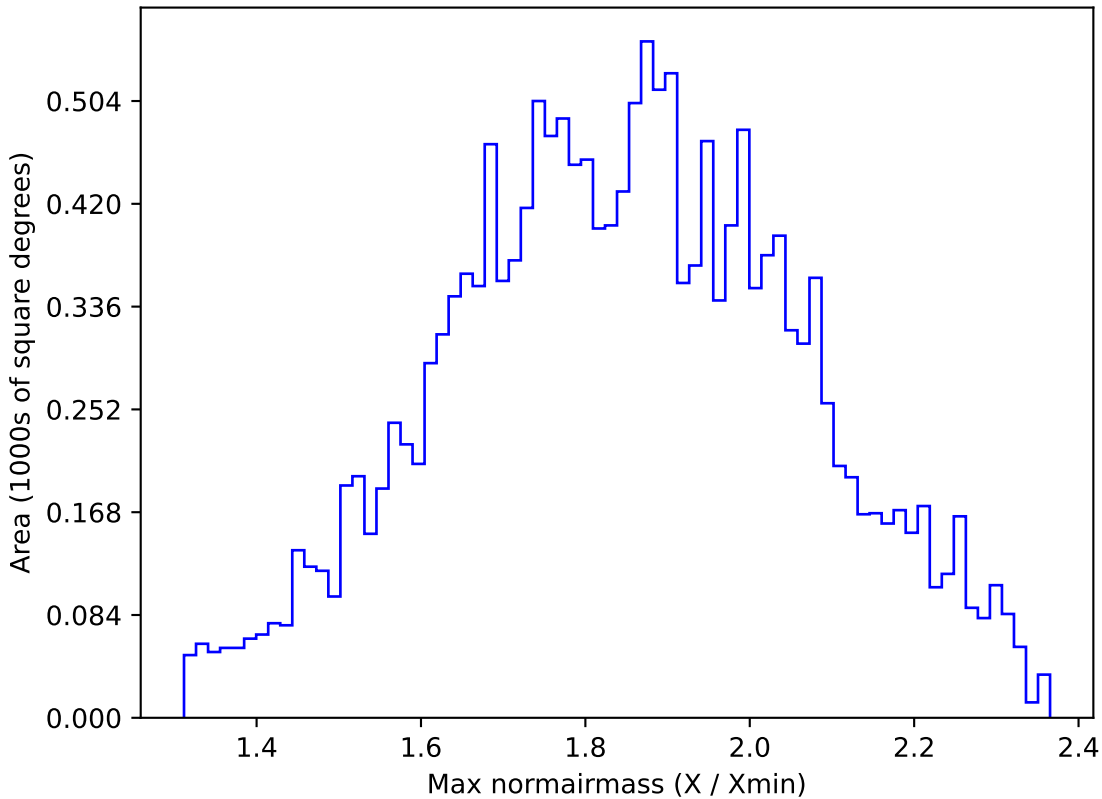
too_elab_r8_d2_griz_v3.4_10yrs WFD g band: Max normairmass
