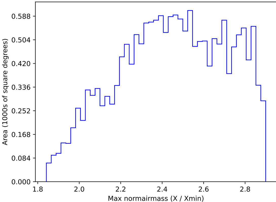
too_elab_r8_d2_griz_v3.4_10yrs WFD all bands: Max normairmass
