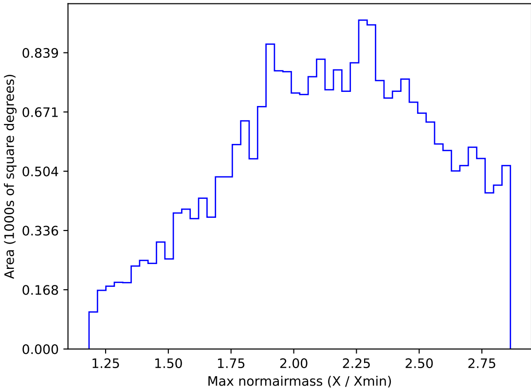
too_elab_r8_d2_griz_v3.4_10yrs All sky z band: Max normairmass
