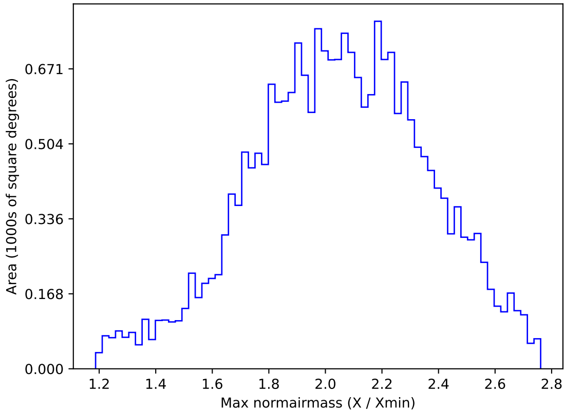
too_elab_r8_d2_griz_v3.4_10yrs All sky y band: Max normairmass
