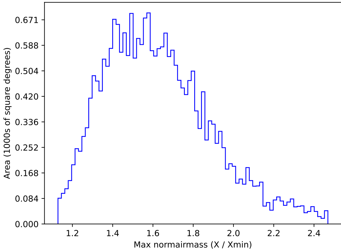
too_elab_r8_d2_griz_v3.4_10yrs All sky u band: Max normairmass
