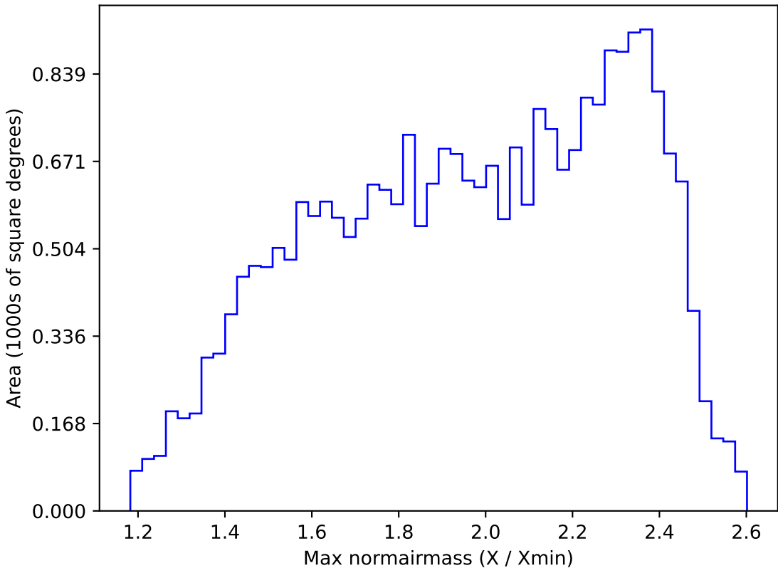
too_elab_r8_d2_griz_v3.4_10yrs All sky r band: Max normairmass
