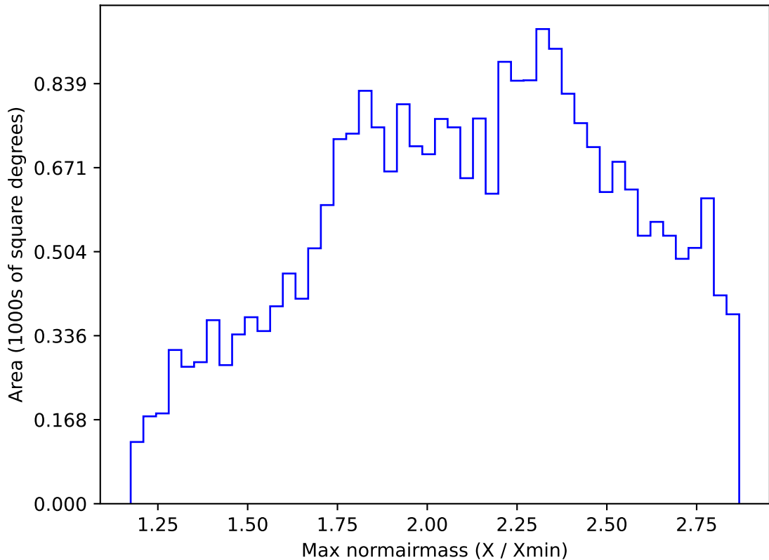
too_elab_r8_d2_griz_v3.4_10yrs All sky i band: Max normairmass
