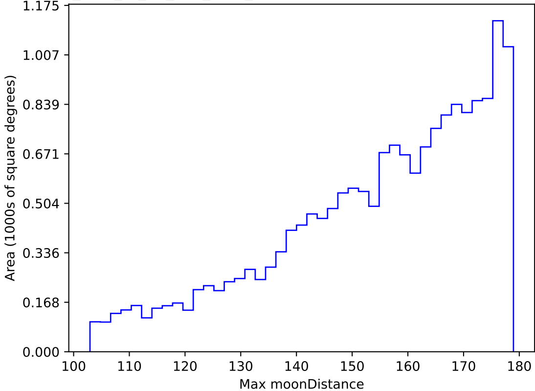
too_elab_r8_d2_griz_v3.4_10yrs WFD z band: Max moonDistance
