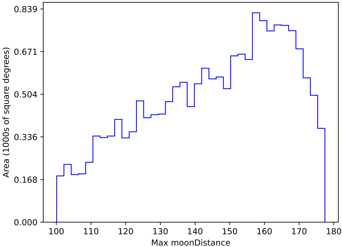
too_elab_r8_d2_griz_v3.4_10yrs WFD y band: Max moonDistance
