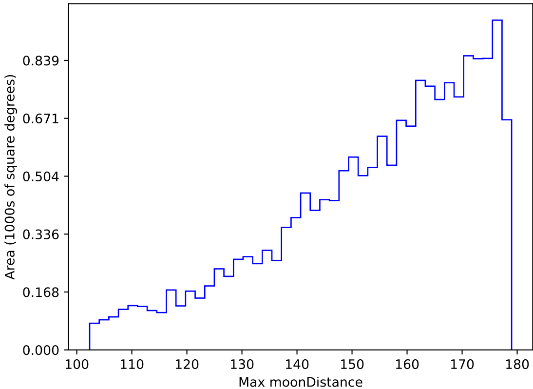
too_elab_r8_d2_griz_v3.4_10yrs WFD u band: Max moonDistance
