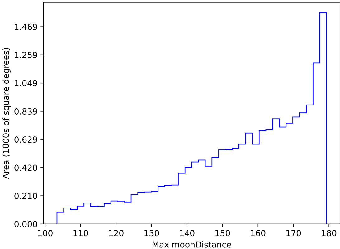
too_elab_r8_d2_griz_v3.4_10yrs WFD r band: Max moonDistance
