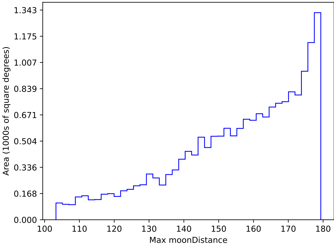
too_elab_r8_d2_griz_v3.4_10yrs WFD i band: Max moonDistance
