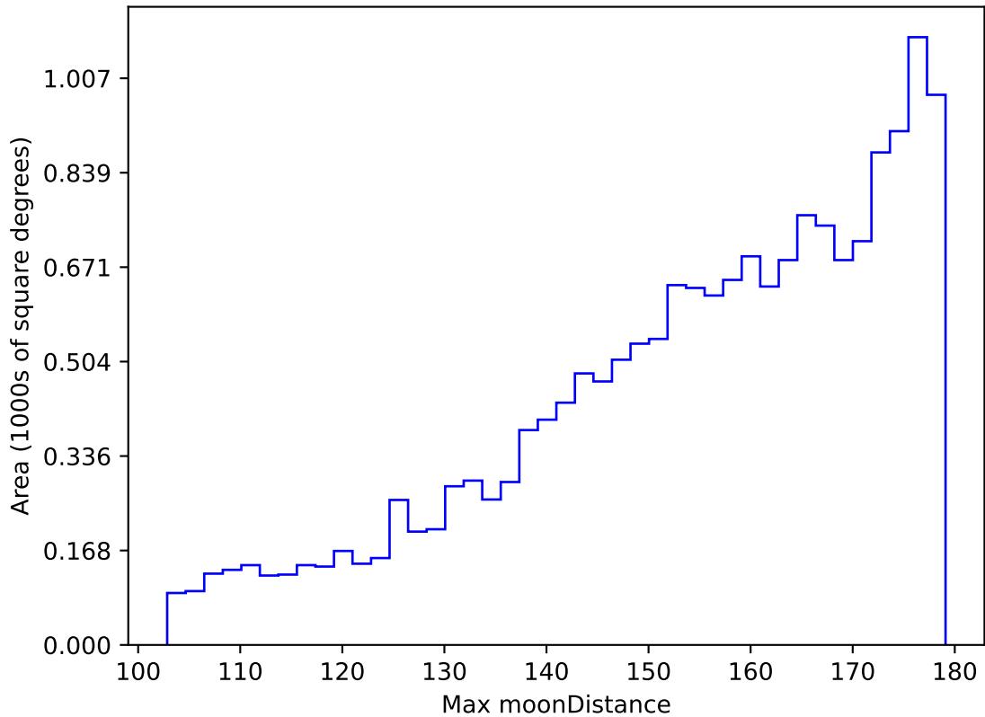
too_elab_r8_d2_griz_v3.4_10yrs WFD g band: Max moonDistance
