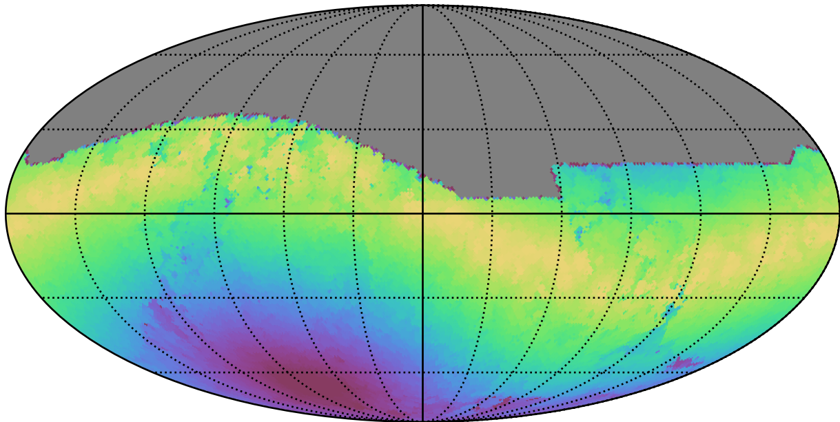
too_elab_r8_d2_griz_v3.4_10yrs All sky z band: Max moonDistance
