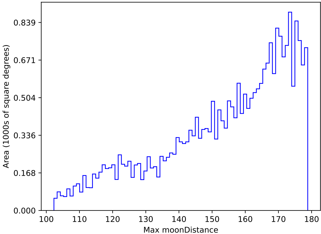
too_elab_r8_d2_griz_v3.4_10yrs All sky z band: Max moonDistance
