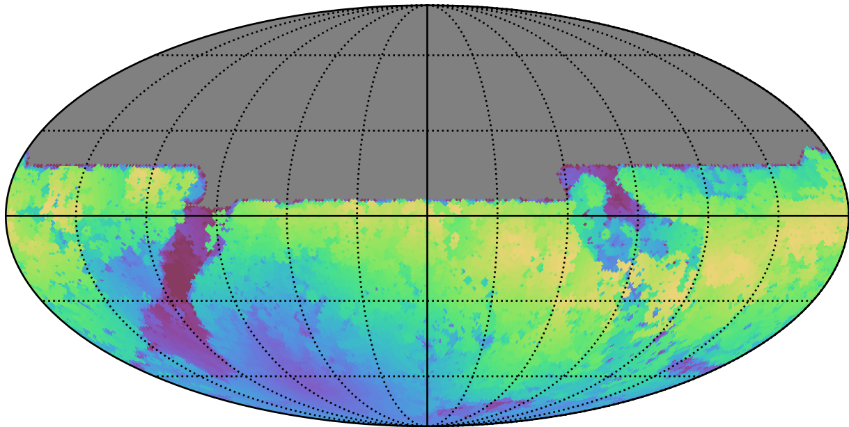
too_elab_r8_d2_griz_v3.4_10yrs All sky y band: Max moonDistance
