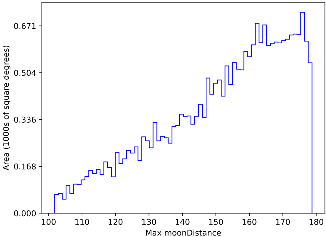
too_elab_r8_d2_griz_v3.4_10yrs All sky u band: Max moonDistance
