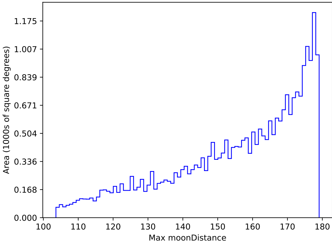
too_elab_r8_d2_griz_v3.4_10yrs All sky i band: Max moonDistance
