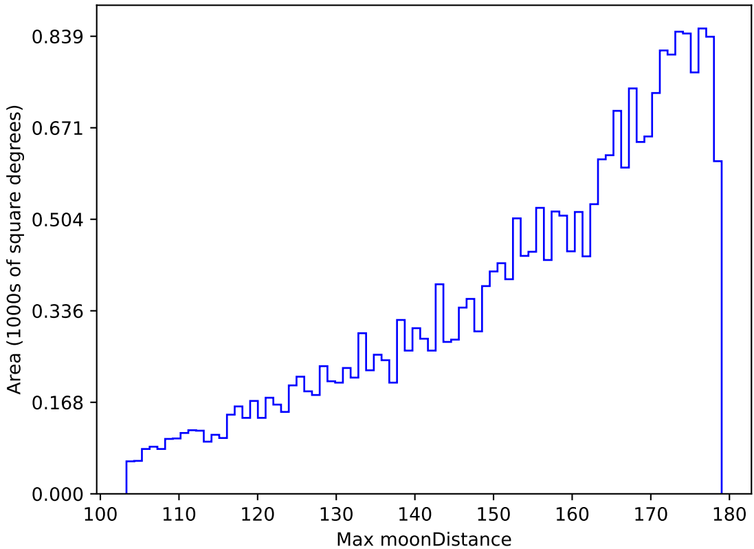
too_elab_r8_d2_griz_v3.4_10yrs All sky g band: Max moonDistance
