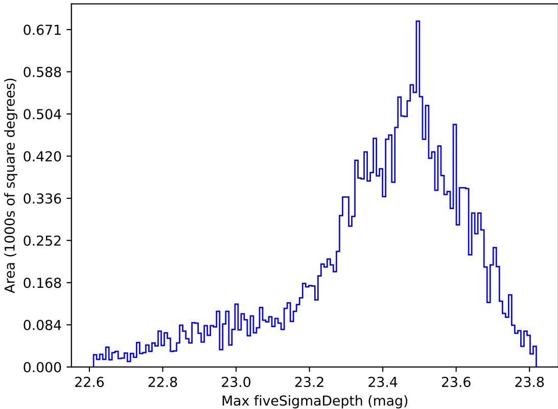
too_elab_r8_d2_griz_v3.4_10yrs Yr 1 z band: Max fiveSigmaDepth
