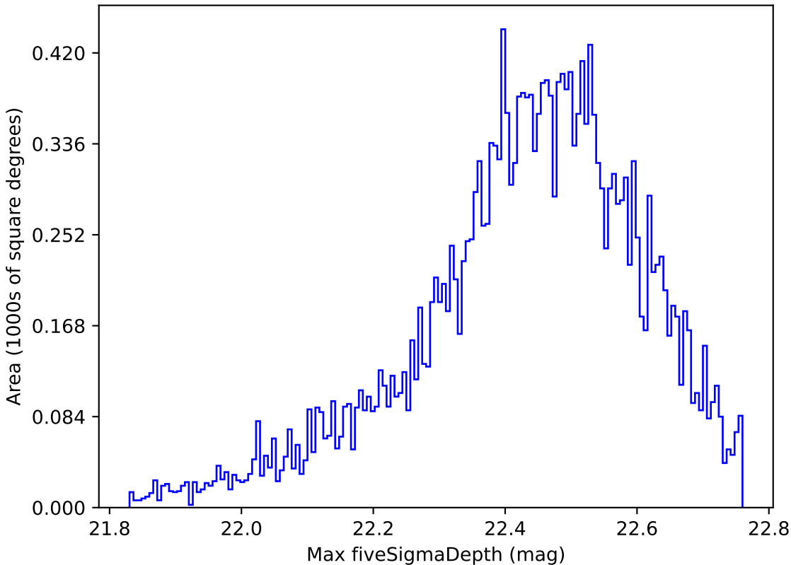
too_elab_r8_d2_griz_v3.4_10yrs Yr 1 y band: Max fiveSigmaDepth
