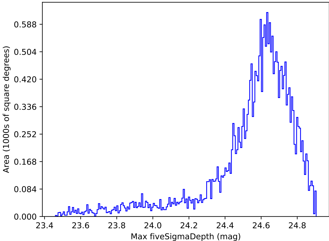
too_elab_r8_d2_griz_v3.4_10yrs Yr 1 r band: Max fiveSigmaDepth
