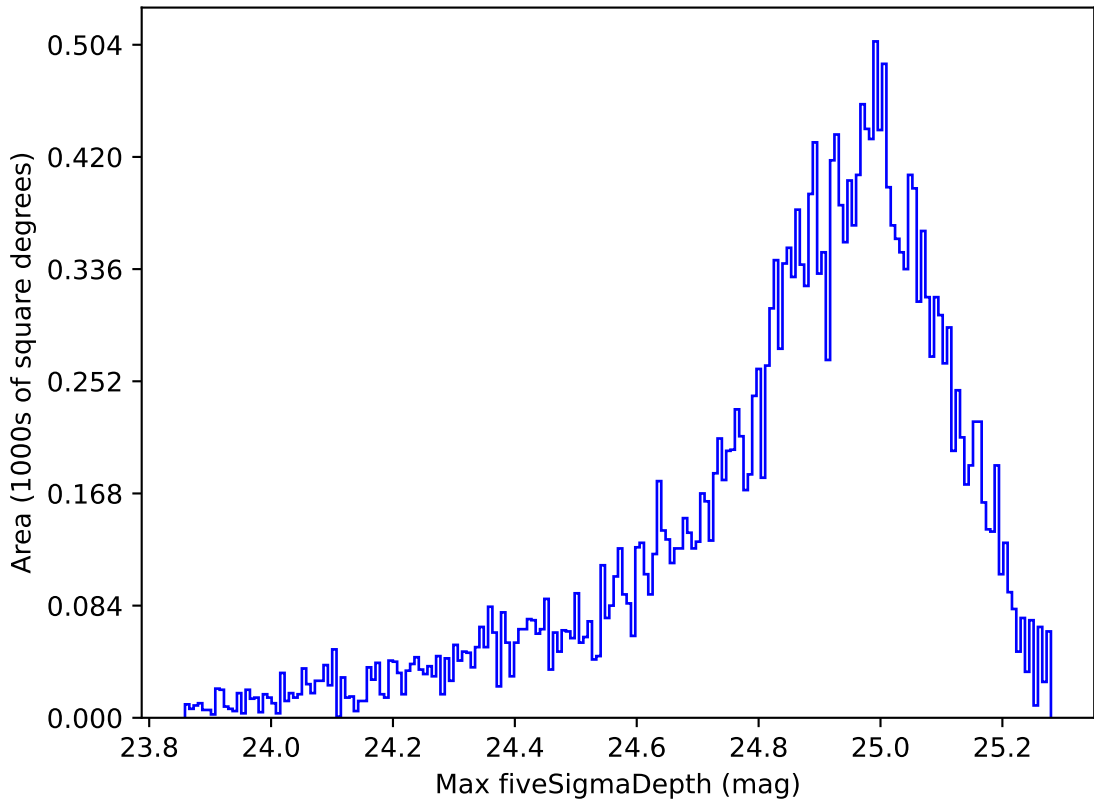
too_elab_r8_d2_griz_v3.4_10yrs Yr 1 all bands: Max fiveSigmaDepth
