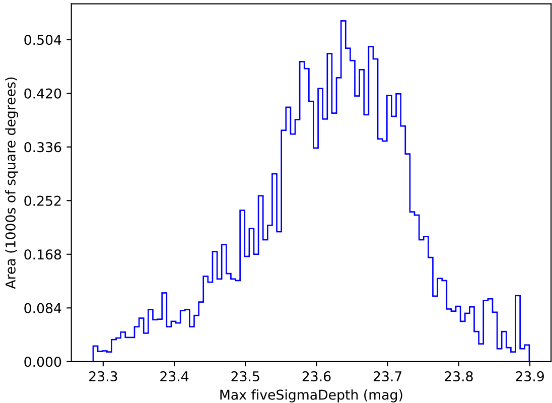
too_elab_r8_d2_griz_v3.4_10yrs WFD z band: Max fiveSigmaDepth
