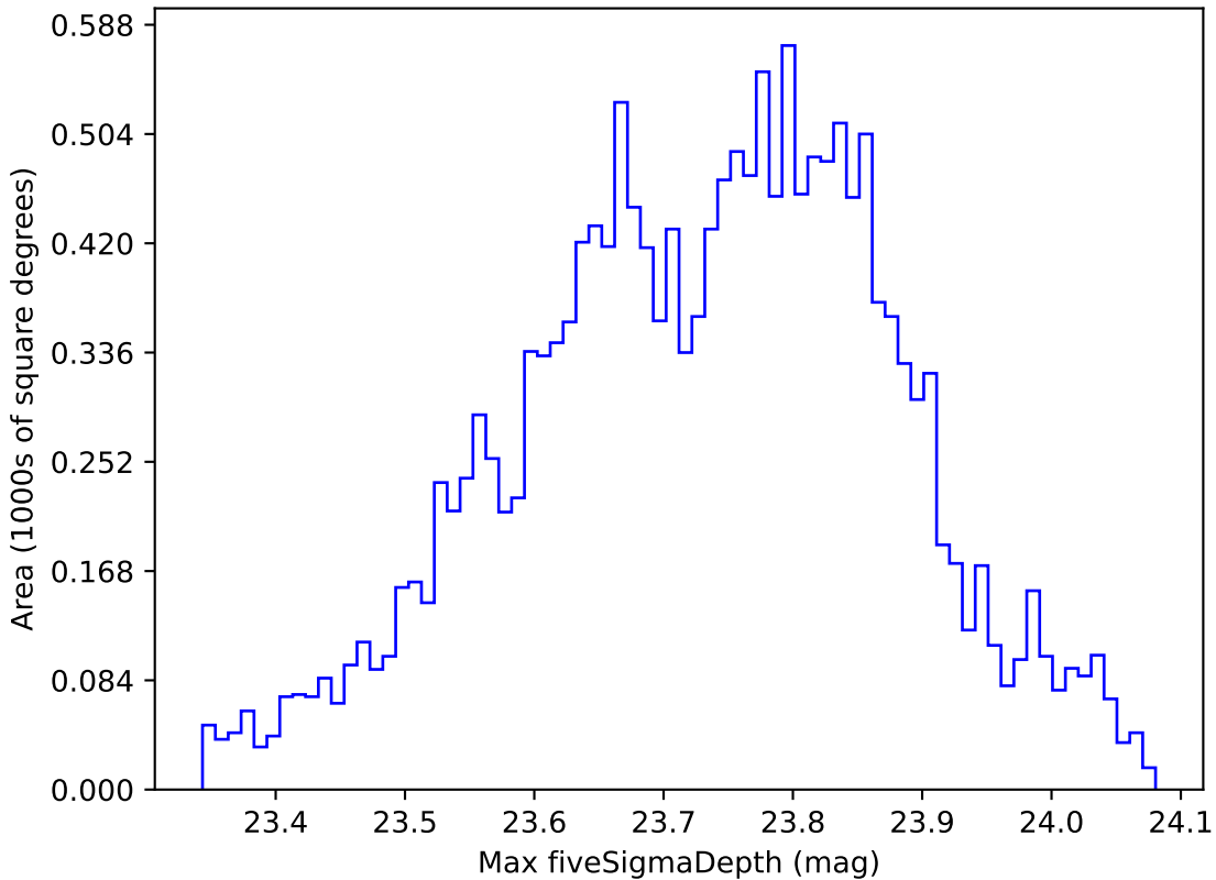
too_elab_r8_d2_griz_v3.4_10yrs WFD u band: Max fiveSigmaDepth
