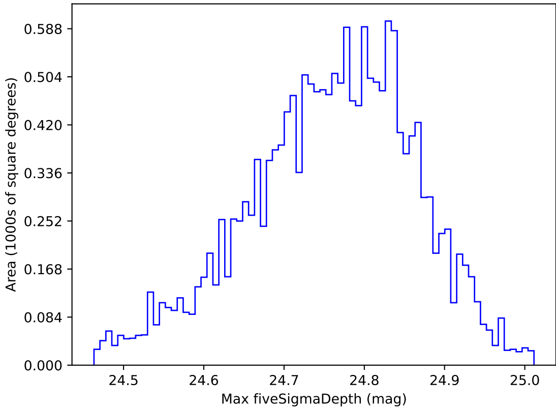
too_elab_r8_d2_griz_v3.4_10yrs WFD r band: Max fiveSigmaDepth
