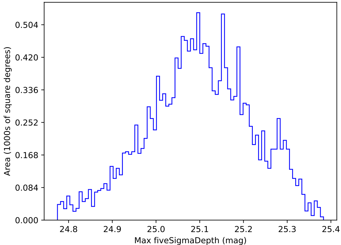
too_elab_r8_d2_griz_v3.4_10yrs WFD g band: Max fiveSigmaDepth
