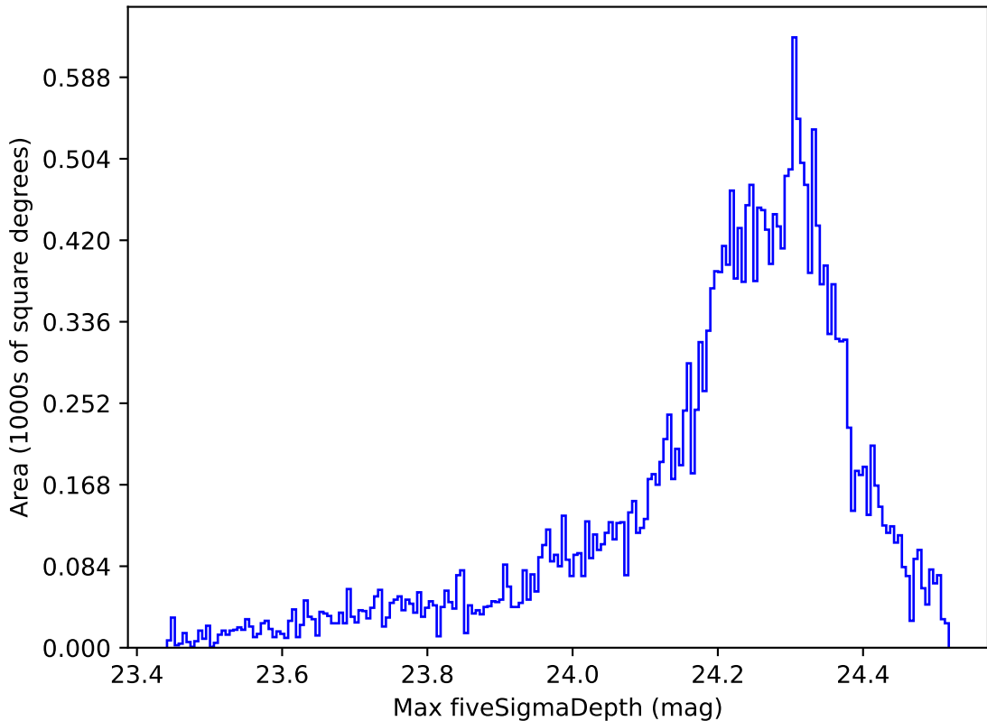
too_elab_r8_d2_griz_v3.4_10yrs All sky i band: Max fiveSigmaDepth
