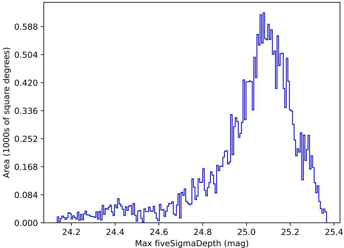
too_elab_r8_d2_griz_v3.4_10yrs All sky g band: Max fiveSigmaDepth
