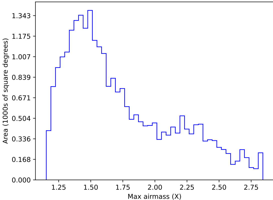
too_elab_r8_d2_griz_v3.4_10yrs Yr 1 z band: Max airmass
