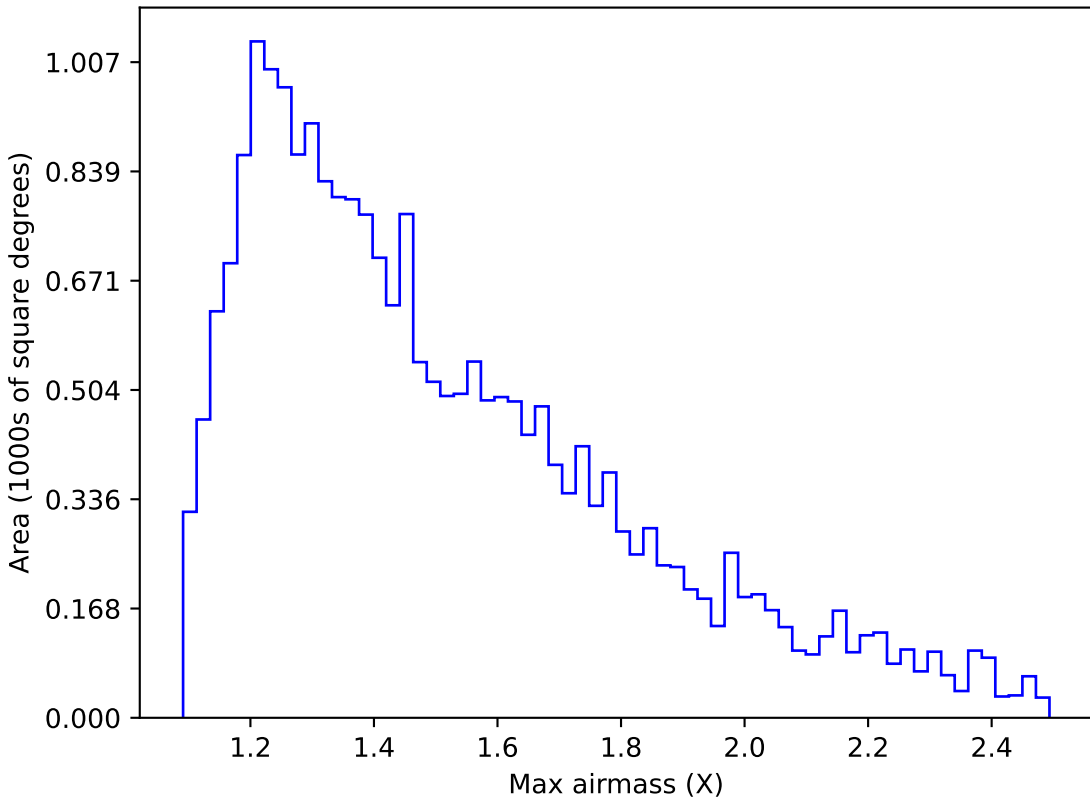
too_elab_r8_d2_griz_v3.4_10yrs Yr 1 u band: Max airmass
