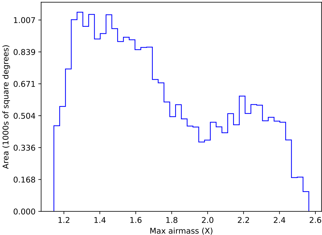
too_elab_r8_d2_griz_v3.4_10yrs Yr 1 r band: Max airmass
