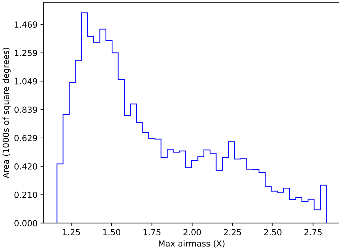
too_elab_r8_d2_griz_v3.4_10yrs Yr 1 i band: Max airmass
