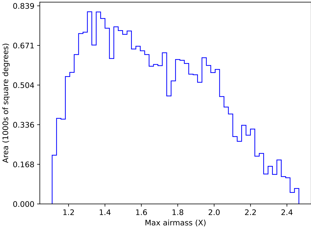
too_elab_r8_d2_griz_v3.4_10yrs Yr 1 g band: Max airmass
